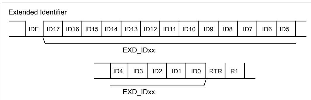
Figure 16-3 Extended identifier
