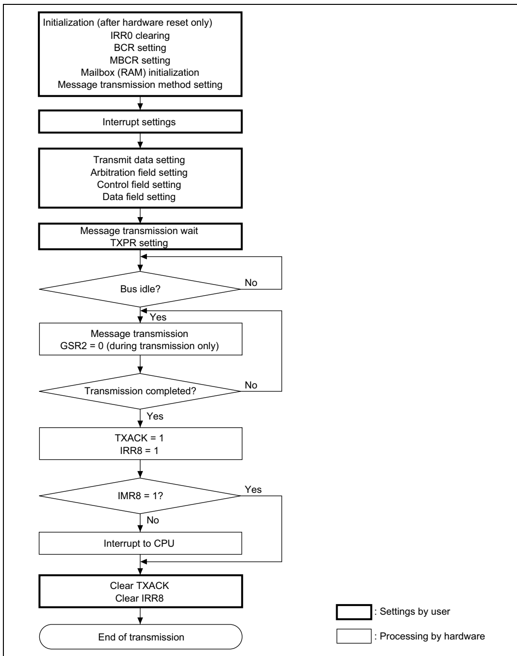
Figure 16-7 Transmission Flowchart
