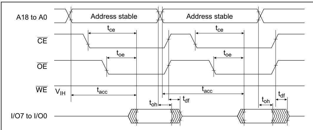
Figure 21A-21 \overline{\text{CE}} and \overline{\text{OE}} Clock System Read Timing Waveforms
