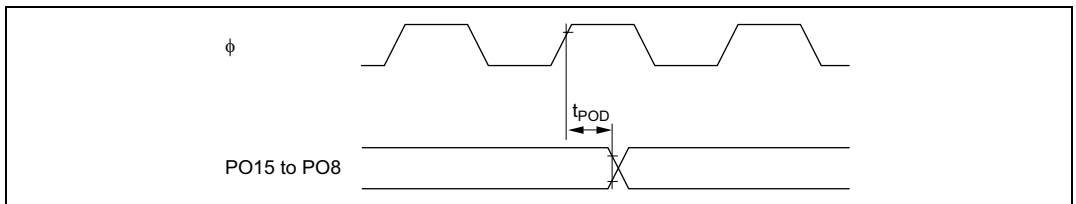
Figure 24-20 PPG Output Timing*
