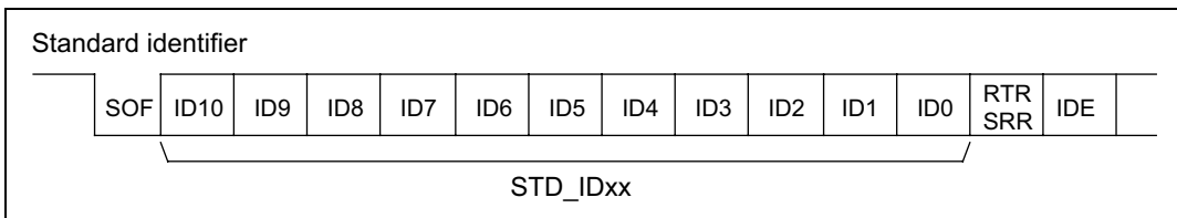
Figure 16-2 Standard identifier
