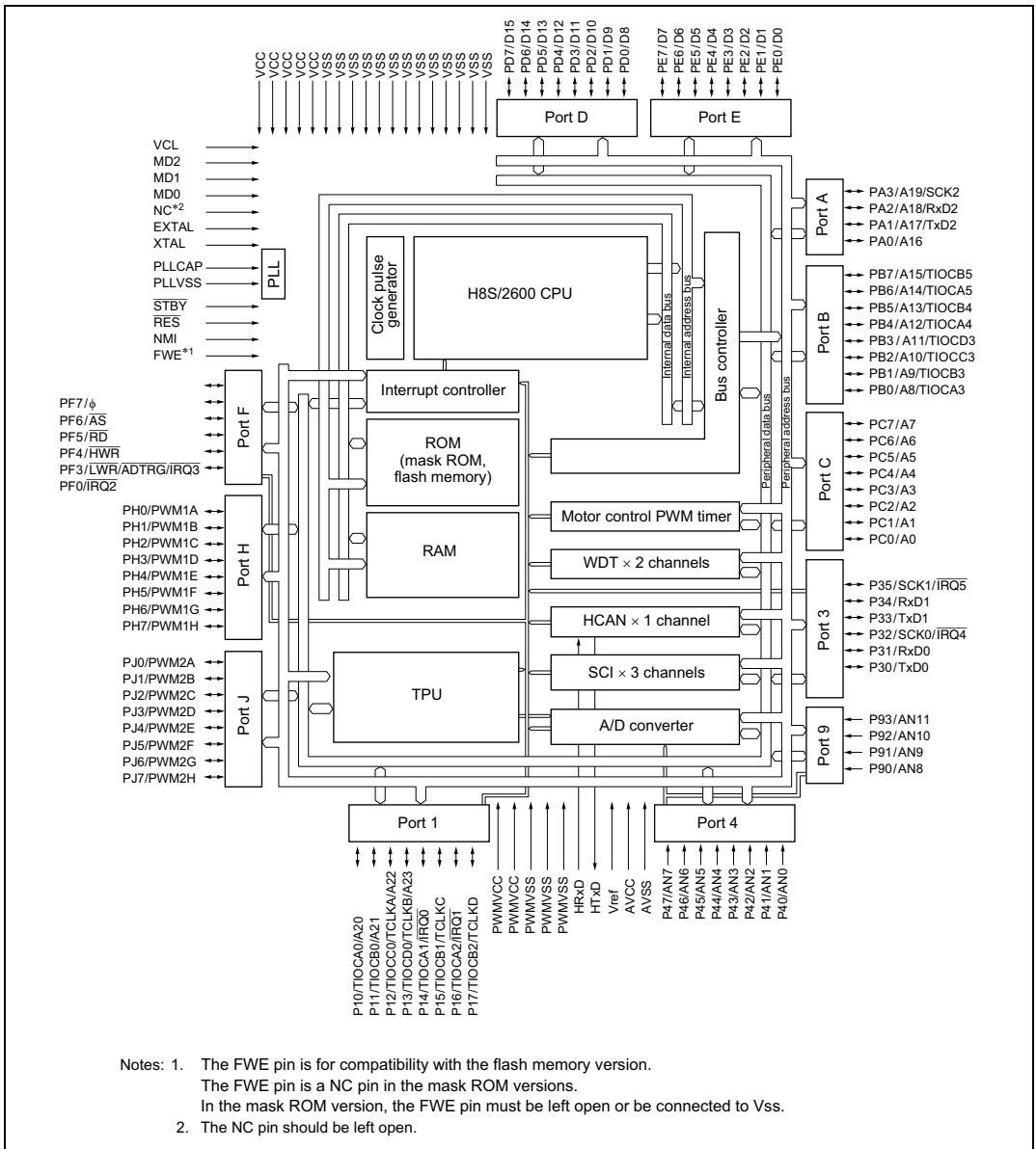
Figure 1-1 (c) shows an internal block diagram of the H8S/2635 Group.
