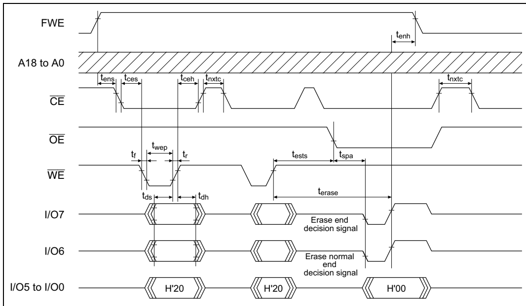
Figure 21C-23 Auto-Erase Mode Timing Waveforms
