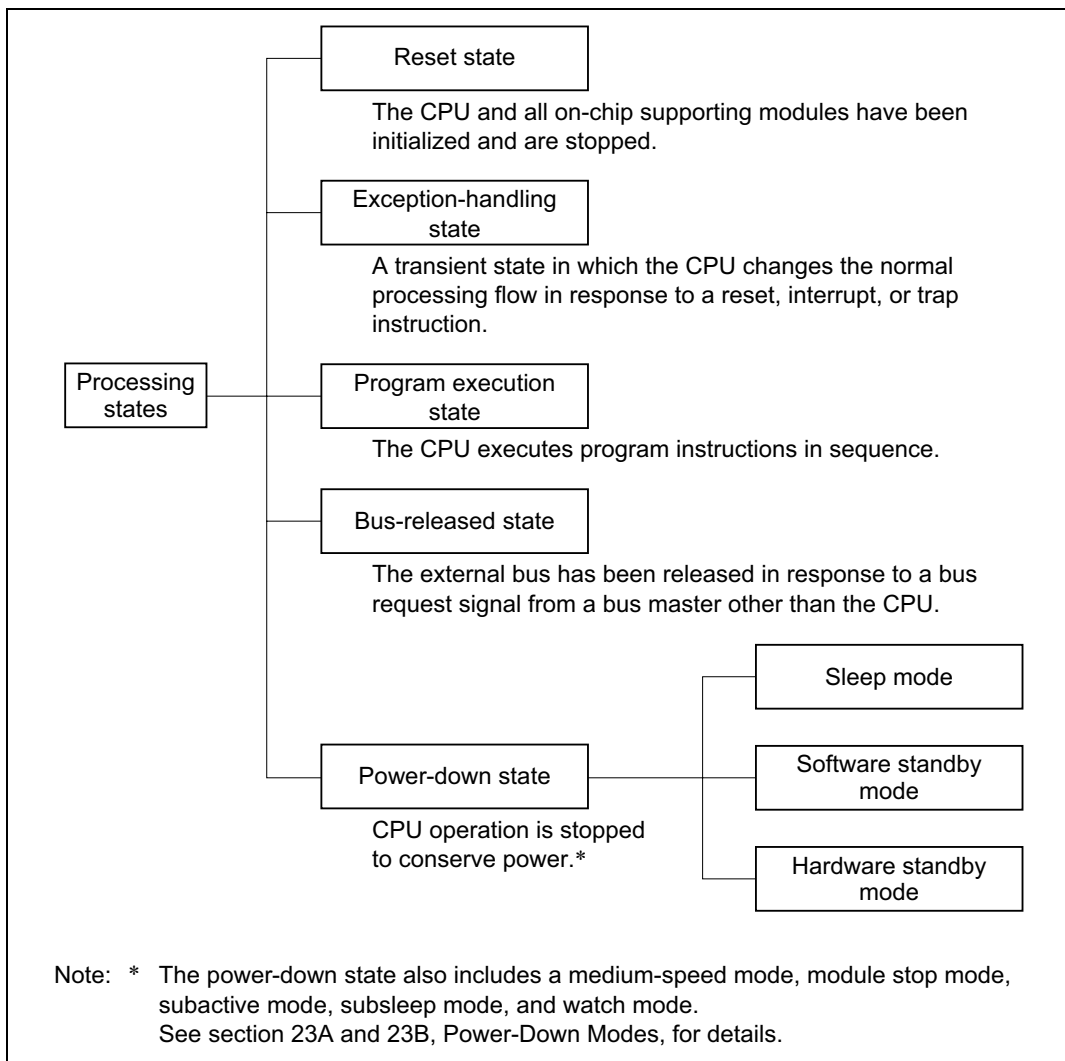
Figure 2-14 Processing States
